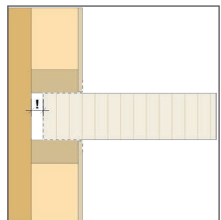
Fig. 4: Structural installation gap
